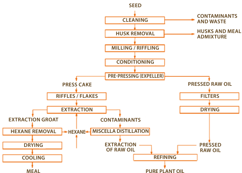
Figure 2 Seed processing in a (centralized) industrial oil mill
